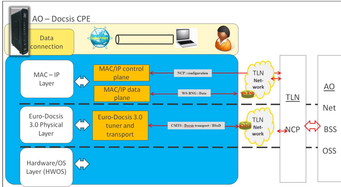
Figure 2-1: AO Euro-Docsis General Overview
