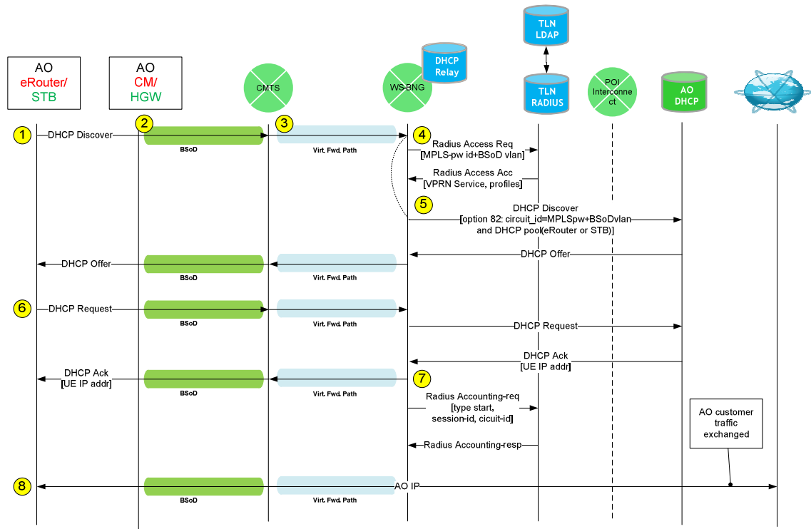
Figure 7-4 : Access Authentication
