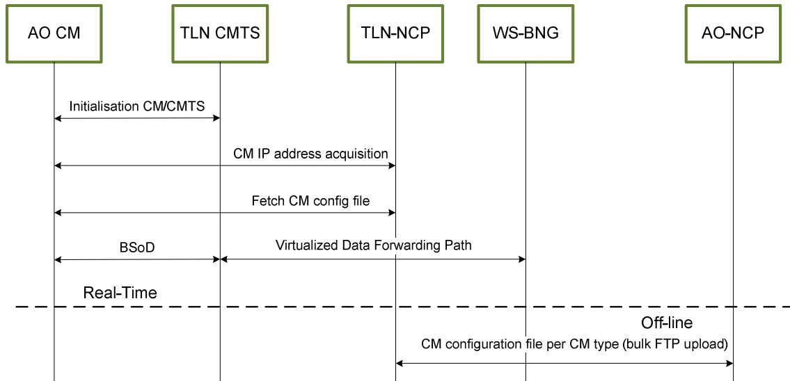
Figure 3-1: CM initialization
